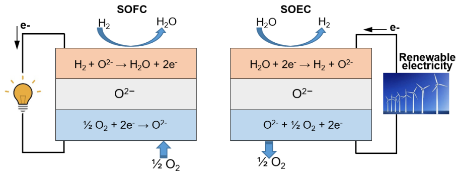
Figure 5.11: Principles of SOEC and SOFC
